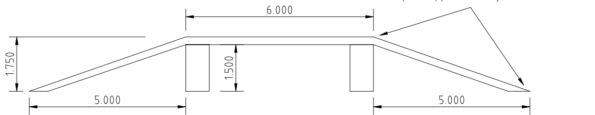
Ramp Side View
