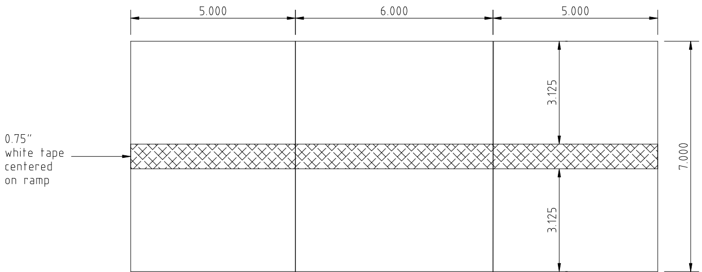
Ramp Top View
