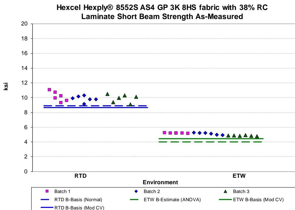
Figure 4-14: Batch plot for SBS1 as-measured
