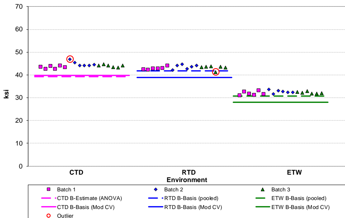
Figure 4-19: Batch plot for FHT2 normalized strength
