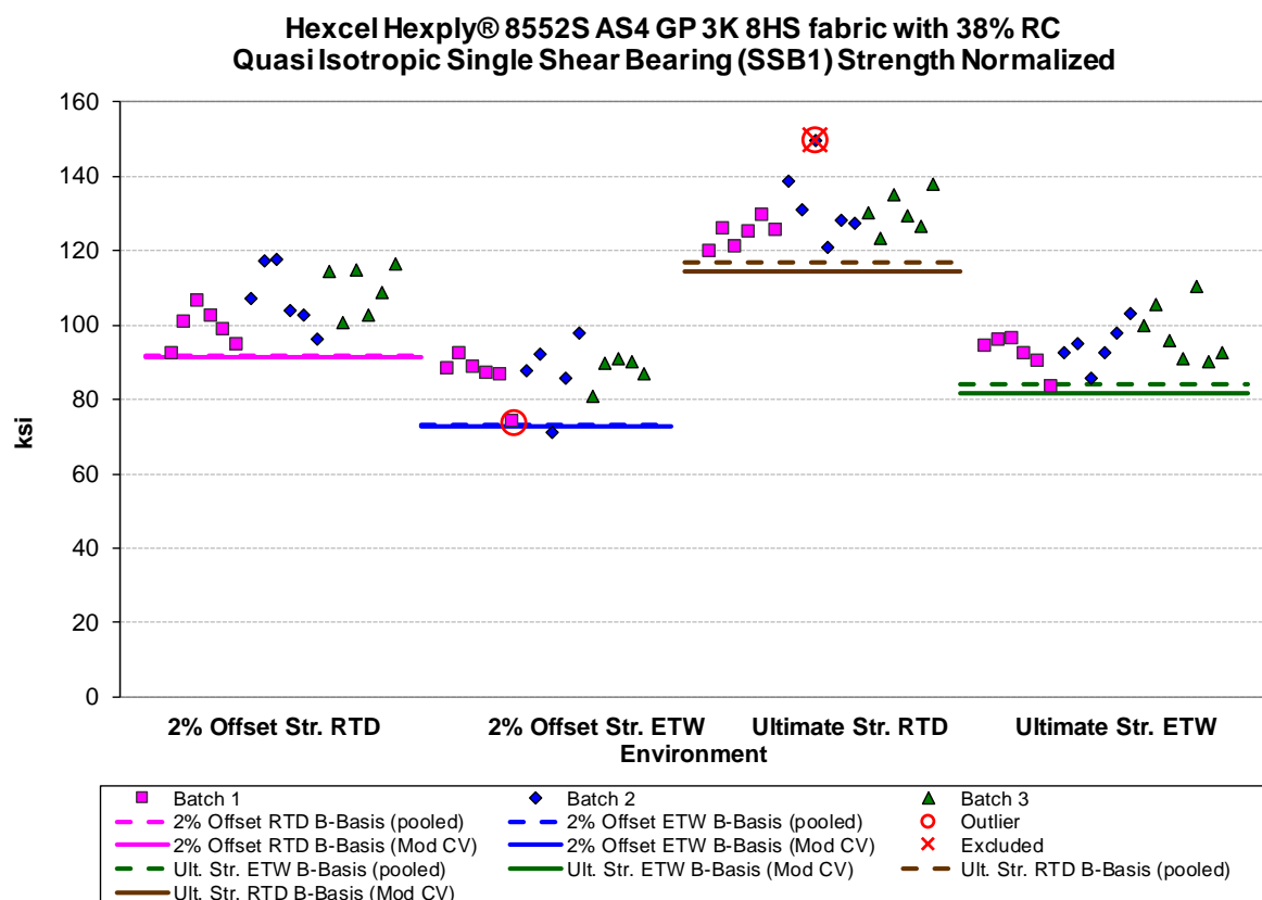
Figure 4-27: Batch plot for SSB1 normalized strength
