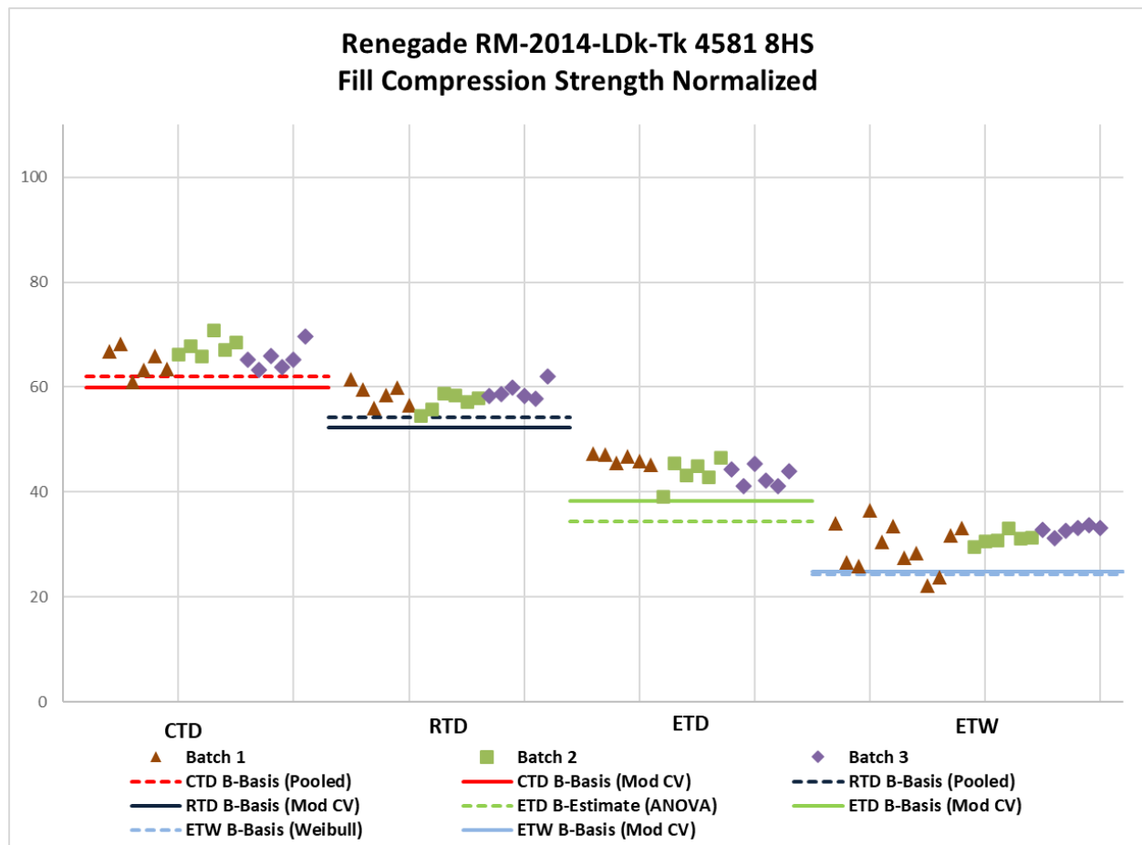
Figure 4-4: Batch Plot for FC Normalized Strength
