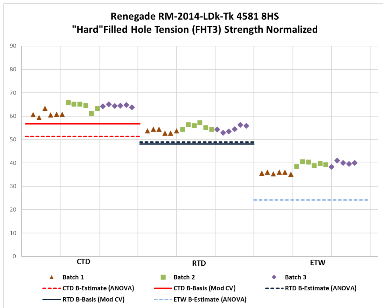
Figure 4-20: Batch plot for FHT3 Normalized Strength
