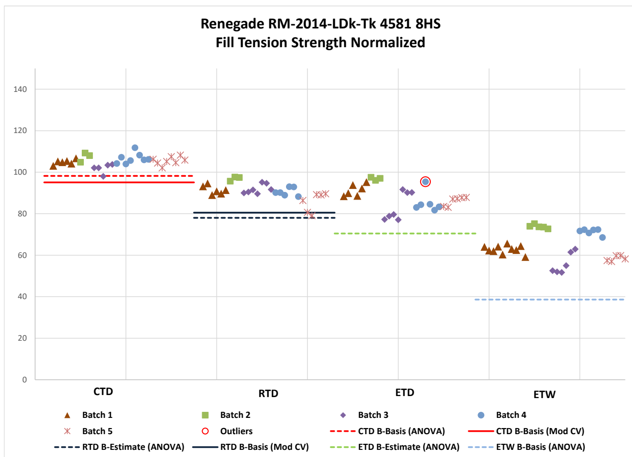
Figure 4-2: Batch Plot for FT Normalized Strength
