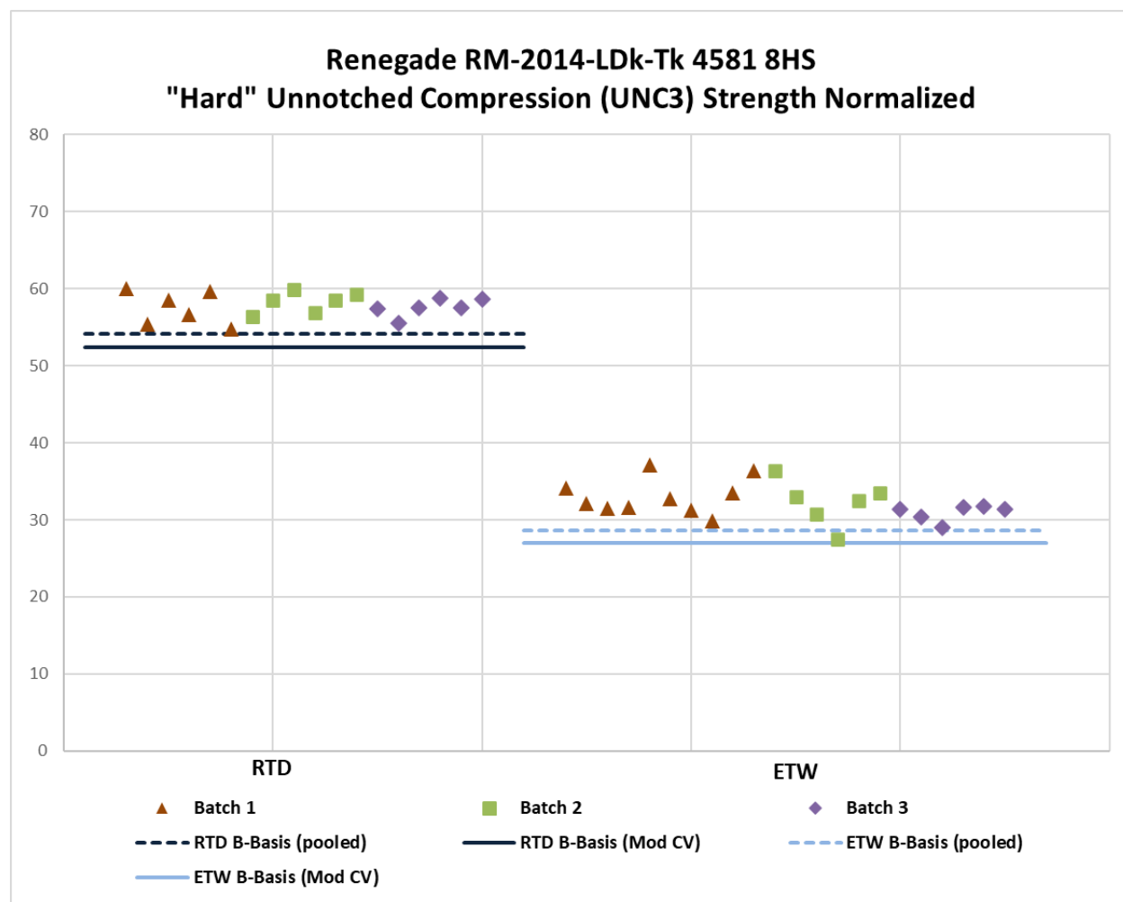
Figure 4-12: Batch Plot for UNC3 Normalized Strength
