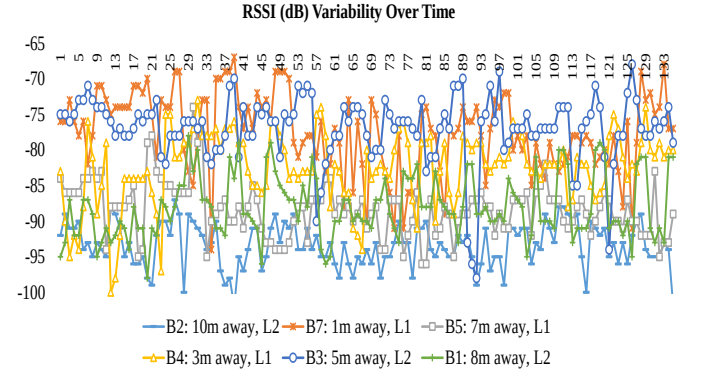
Fig. 1: Variability of RSSI for six beacons placed at different distances away. Beacons are labeled B1, B2, B3, B4, B5, and B7 and these are either on level 1 (L1) or level 2 (L2) of the building represented in Figure 3.
