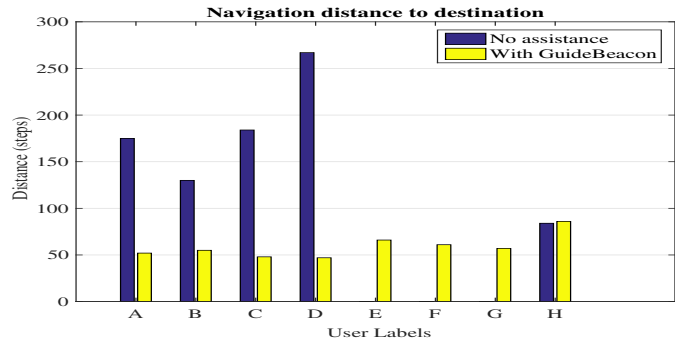
Fig. 7: Navigation distance
