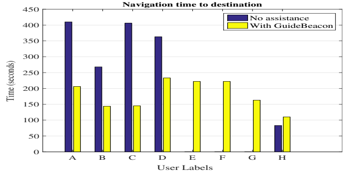
Fig. 6: Navigation time
